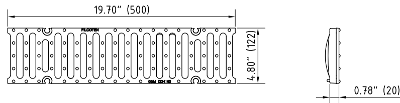
F900kN SW14/100: GJS 17010107, 4-point bolting
