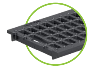
mesh grating NW 150 MW 15/28, class C, ductile iron
