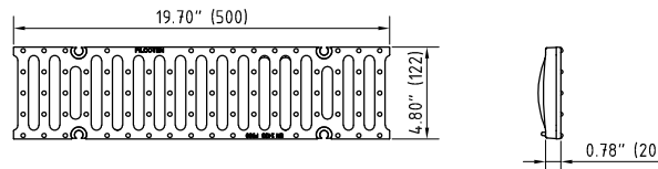
F900kN SW14/100: GJS 17010107, 4-point bolting
