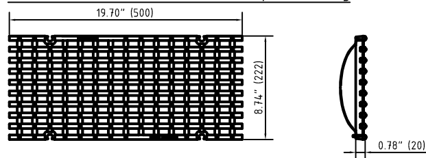
E600kN MW22/13: GJS 17020103, 4-point bolting
