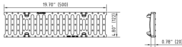
E600kN SW14/100: GJS 17010105
