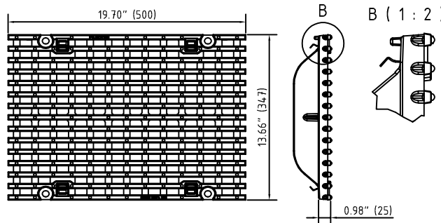
E600kN MW29/13: GJS 17030103
