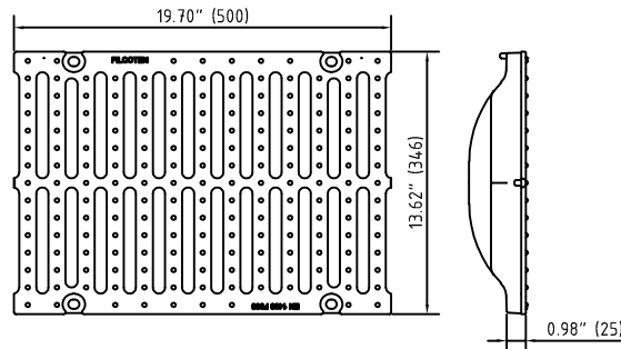
F900kN SW2x16/140: GJS 17030107, 4-times bolted
