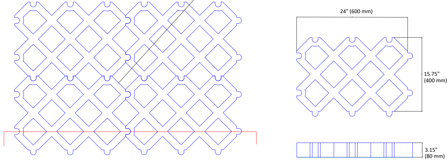
citygrid 3.15" (80 mm) deep Extra heavy Duty grass/gravel reinforcement unit (porous paving grid). Scale: N.T.S
