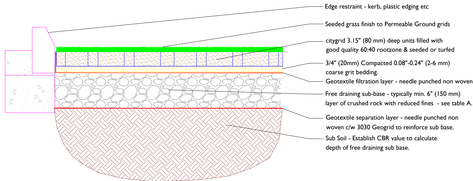
citygrid 3.15" (80 mm) deep Extra heavy Duty grass/gravel reinforcement unit (porous paving grid). Scale: N.T.S
